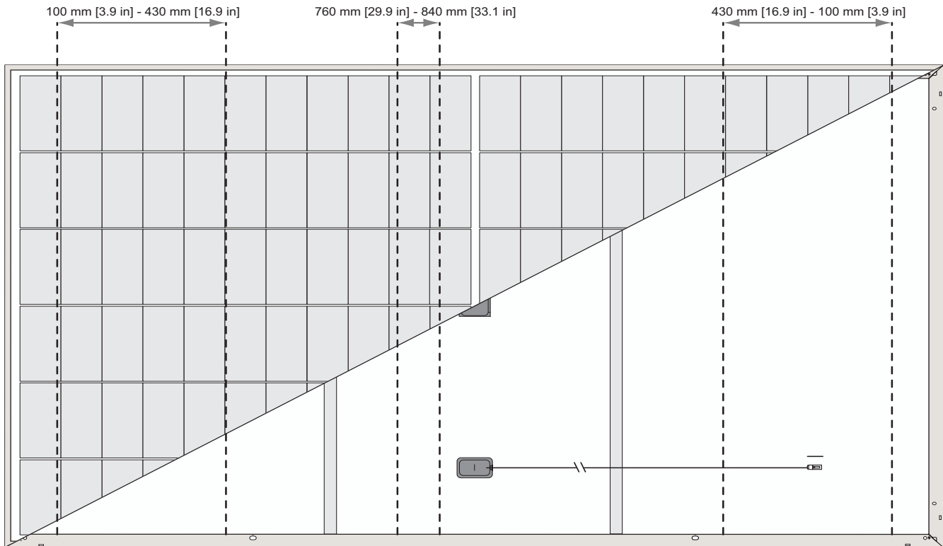
Fig. 24: Six-point mounting configuration clamping zones
