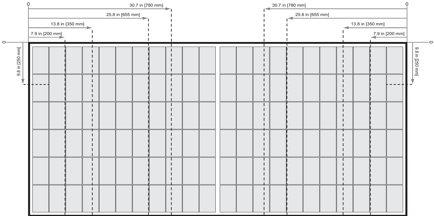
Fig. 9: Clamping of REC Alpha 72 Series panels with rails parallel to short side of the panel
