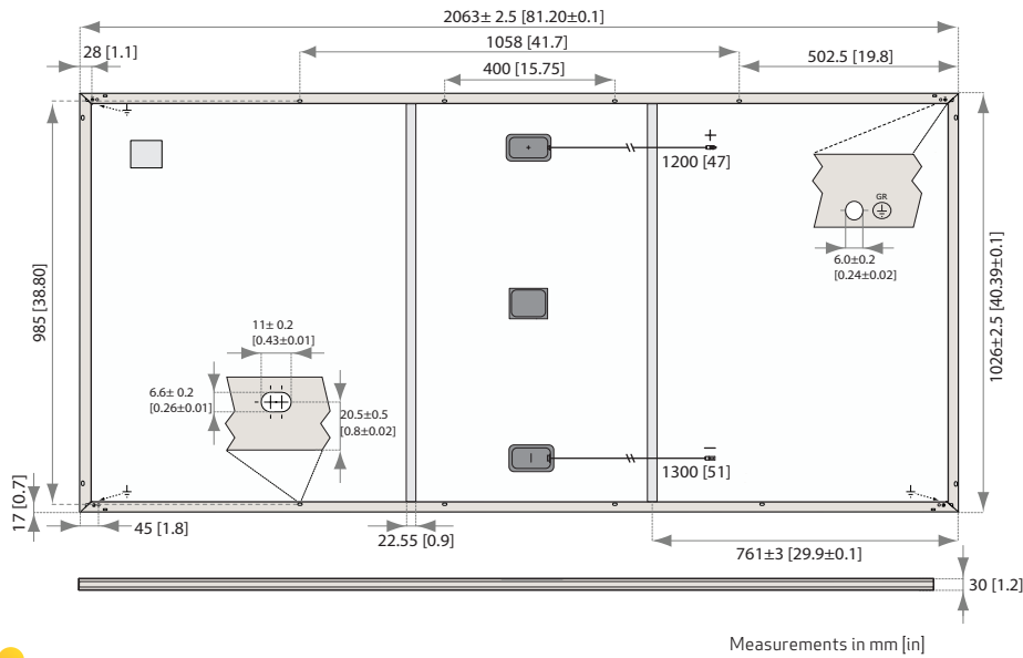
Fig. 21: Panel dimensions: REC Alpha 72 Series
