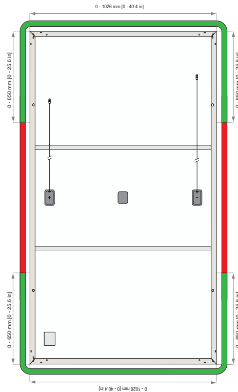
Fig. 23: REC Alpha 72 Series MLPE device installation zones
