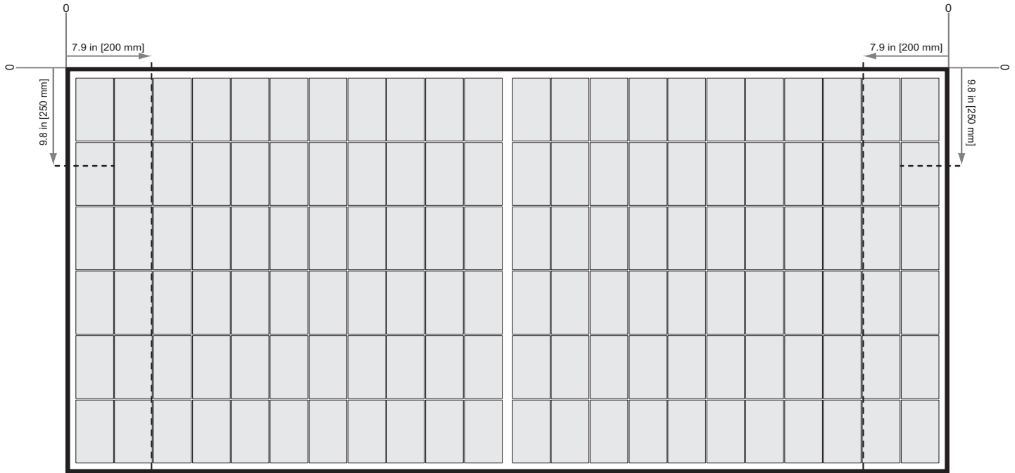
Fig. 10: Clamping of REC Alpha 72 Series panels using short rails
