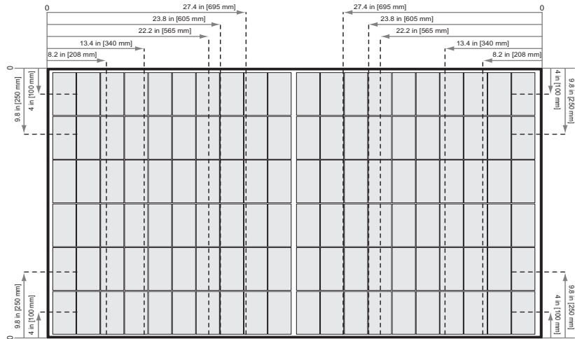
Fig. 5: Clamping of REC Alpha Series panels using a short support
