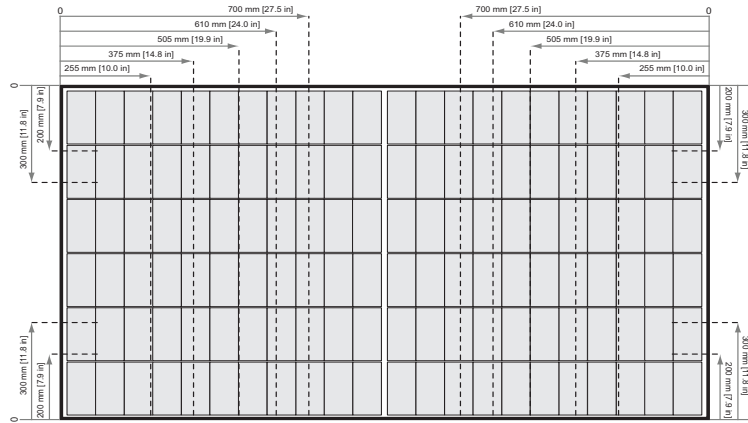
Fig. 8: Clamping of REC Alpha Pure Series panels using short rails
