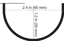
Fig. 17: Minimum cable bend radius
