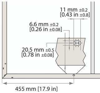
Fig. 11: Mounting holes: REC Alpha Series
