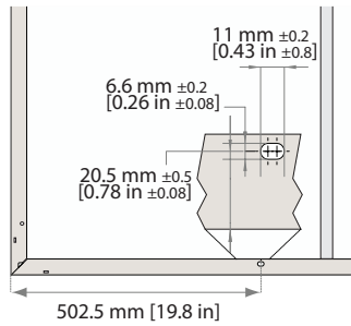
Fig. 12: Mounting holes: REC Alpha 72 Series
