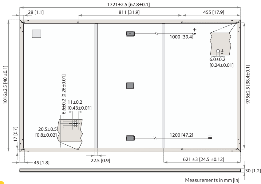
Fig. 19: Panel dimensions: REC Alpha Black Series
